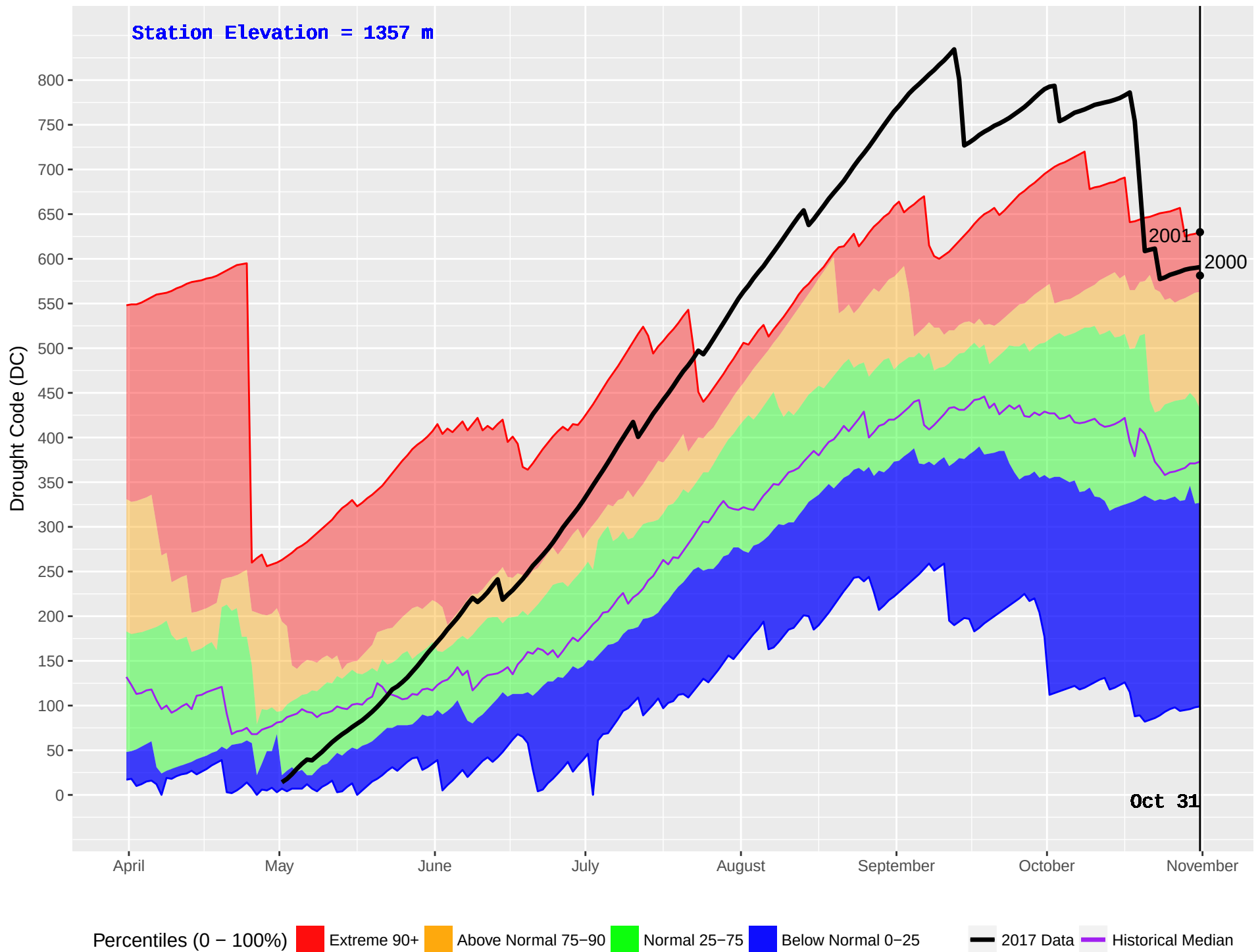
WHITE RIVER (790) : Historical (1989–2016) and Current (2017) Noon Drought Code (DC)
