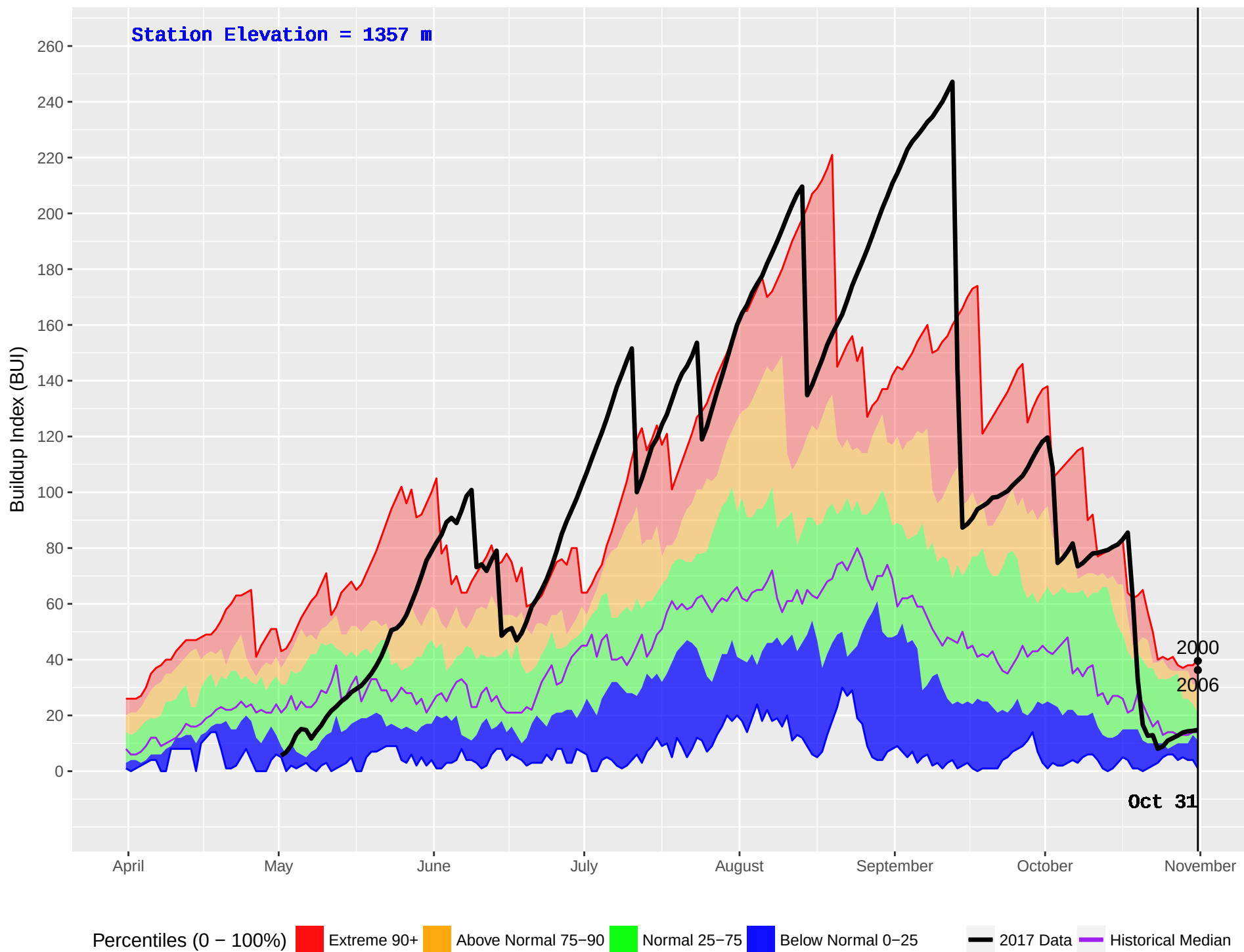
WHITE RIVER (790) : Historical (1989–2016) and Current (2017) Noon Buildup Index (BUI)
