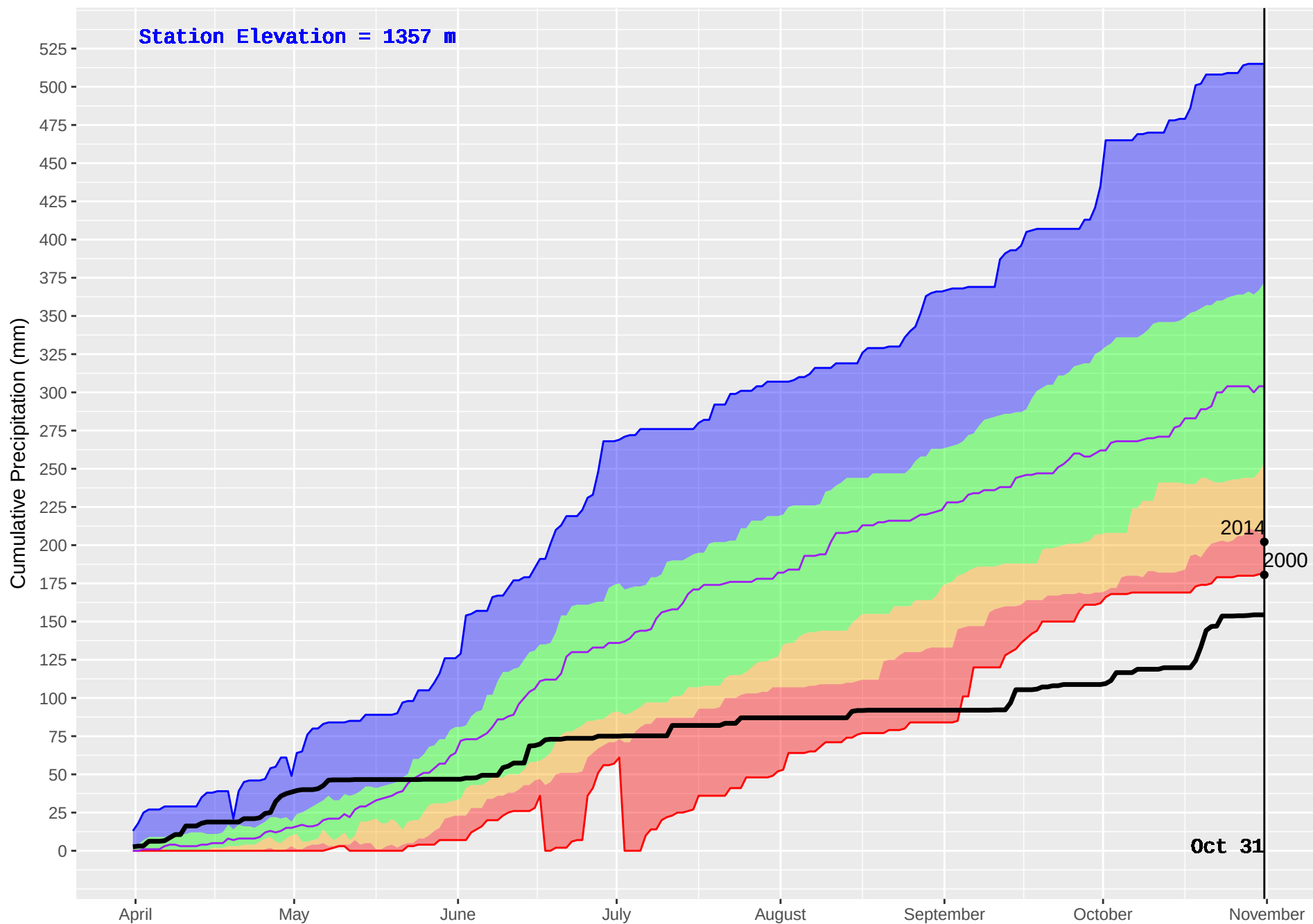
WHITE RIVER (790) : Historical (1989–2016) and Current (2017) Noon Cumulative Precipitation
